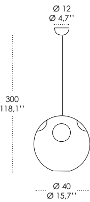
LD0517 1+3 luci/1+3 light
