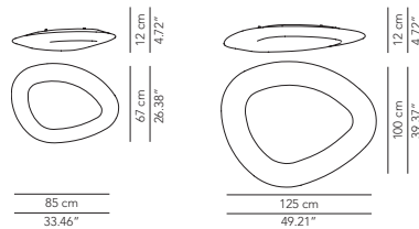
Ceiling-wall lamp
