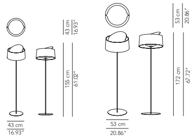
Floor lamp
